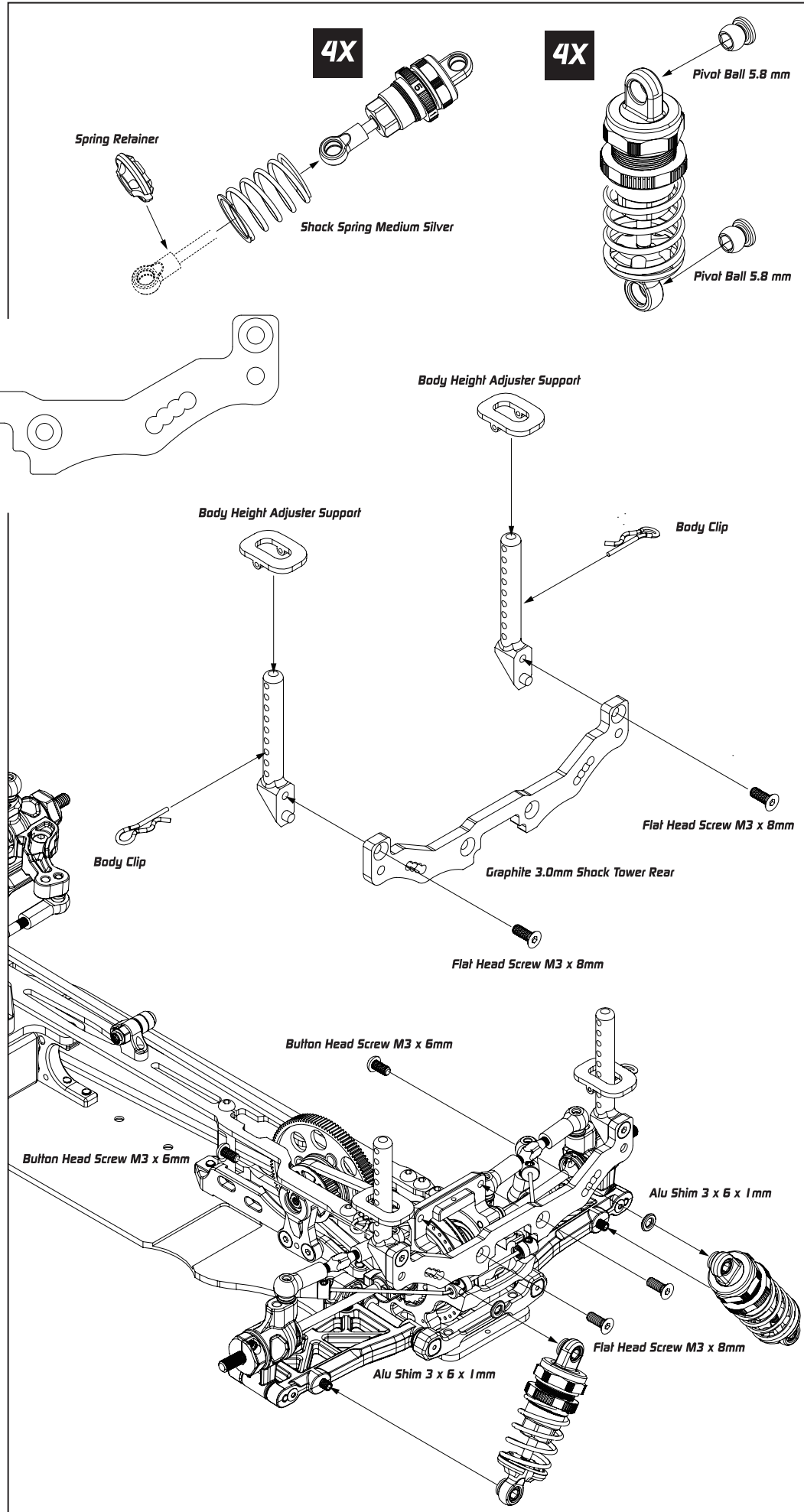
Shock Spring Medium Silver XP-10169
