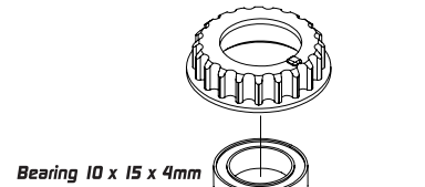
Composite Adjustment Ball-Bearing Hub
