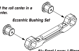
Alu Front Lower 1-Piece Suspension Holder - FF
