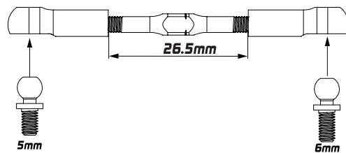
Turnbuckle M3 x 39mm
