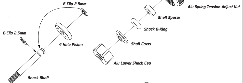
Alu Spring Tension Adjust Nut
